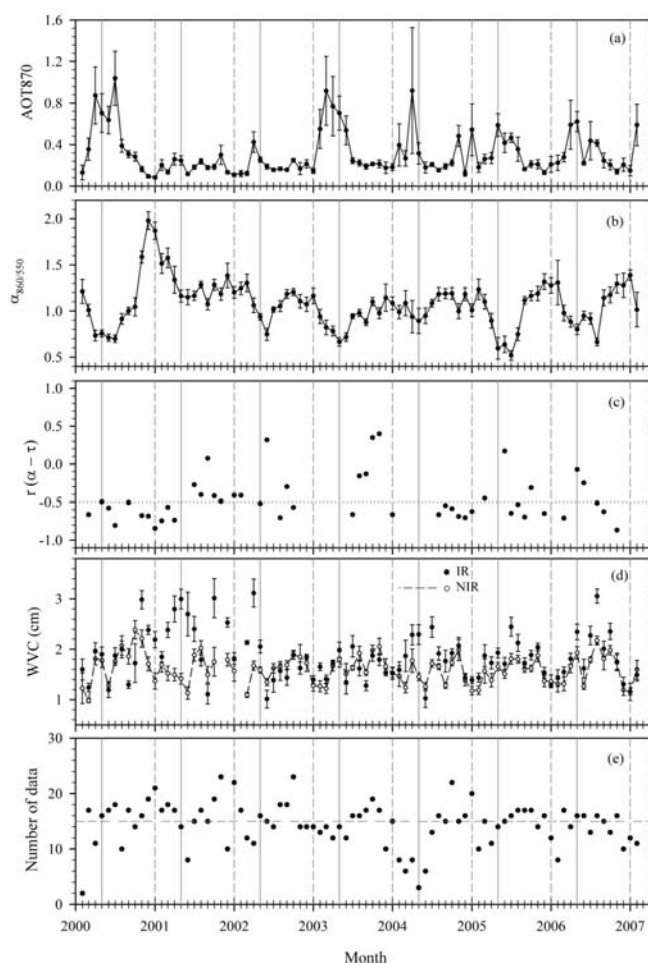
Figure 1. Time series of the monthly mean values of: (a) AOT at 870 nm, (b) Angstrom exponent, (c) correlation coefficients between the daily values of AOT and \alpha for the months with \geq 15 days of data, (d) water vapor content observed at IR (closed circles) and NIR (open circles), (e) number of days used in each year. Vertical solid lines represent the month of Mays, while vertical dashed lines represent the month of Januarys.
