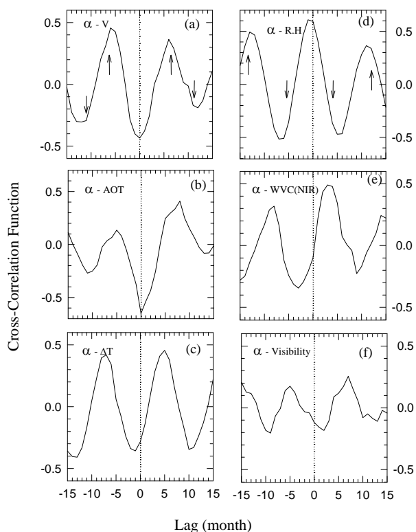
Figure 4. Cross-correlation functions versus time lag between the Angstrom exponent \alpha and: (a) wind speed, V ; (b) AOT (c) diurnal temperature range, \Delta T (d) relative humidity, RH ; (e) water vapor content, WVC observed at NIR; (f) visibility.
