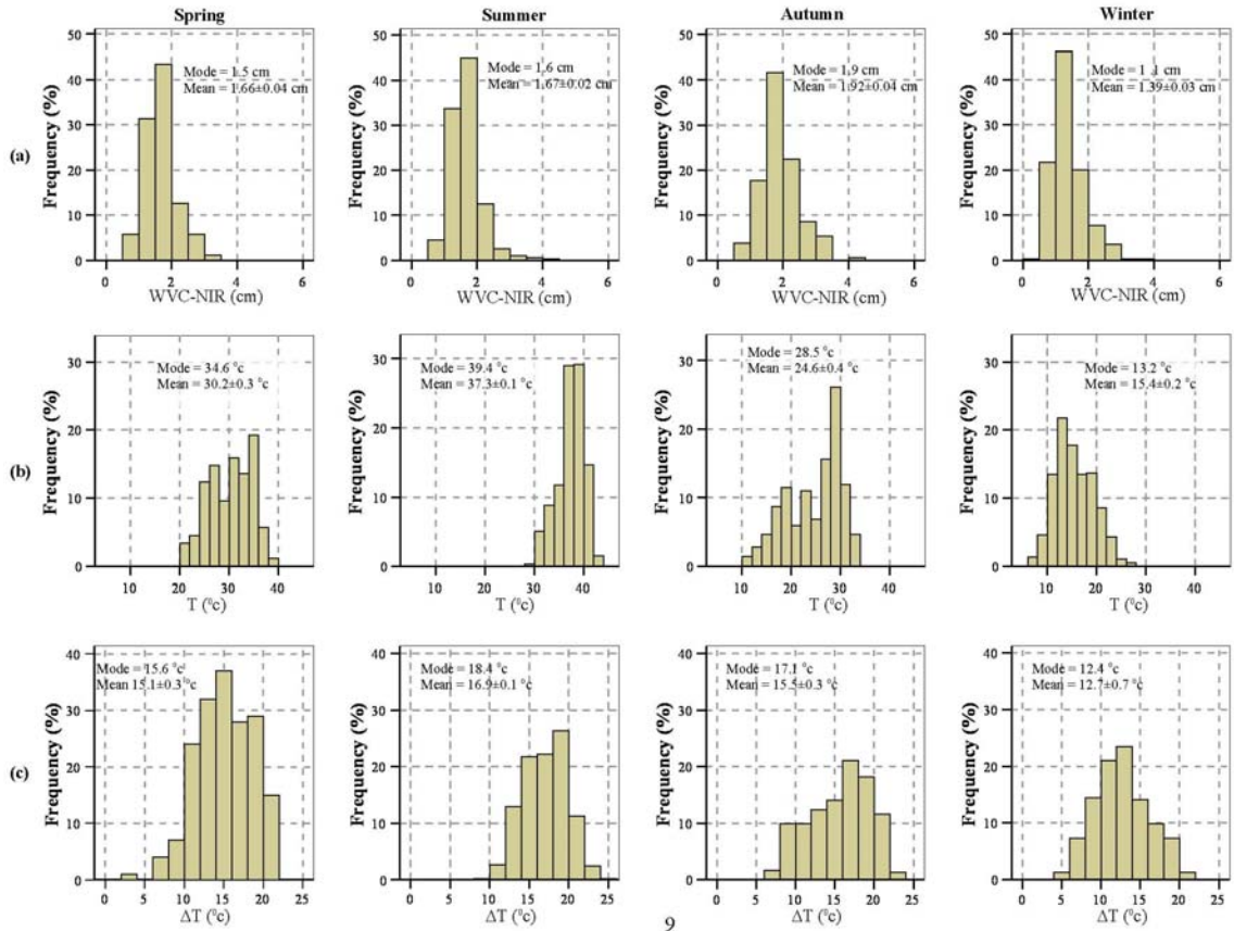
Figure 6. Same as for Figure 4 but for: (a) water vapor content (NIR), (b) air temperature, (c) the diurnal temperature range.
